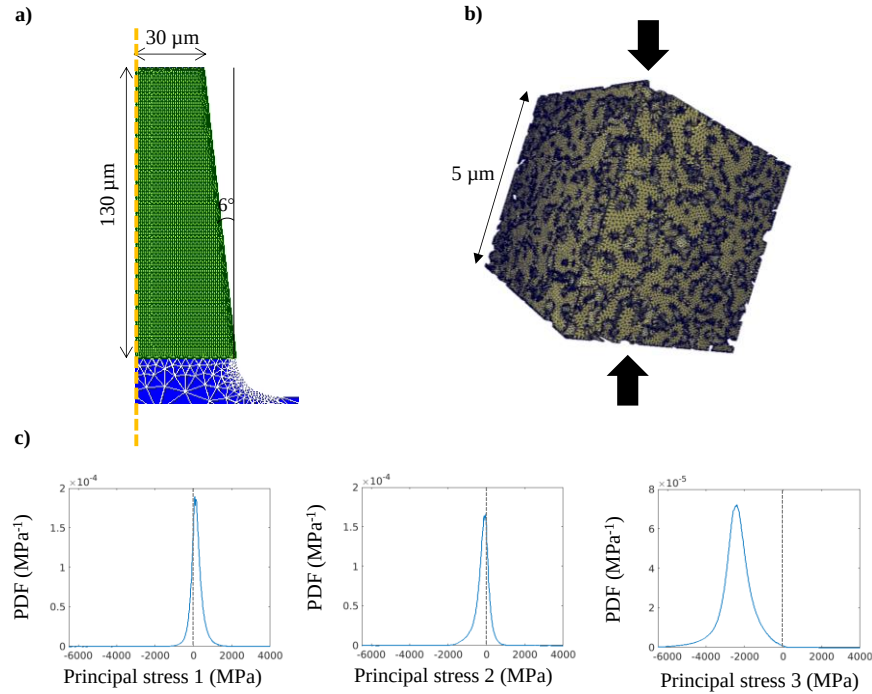
Fig11. Multiscale approach: a) axisymmetric geometry of the micro-pillar, b) porous YSZ microstructure under compression, c) probability density function (PDF) of the principal stresses.
